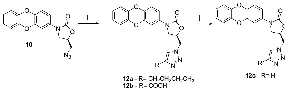
Scheme 2. Reagents and condition: (i) sodium ascorbate, CuSO_4 \cdot 5H_2O , t -BuOH/ H_2O , for 12a : 1-hexyne, for 12b : propionic acid; (j) from 12b , DMF, reflux.
